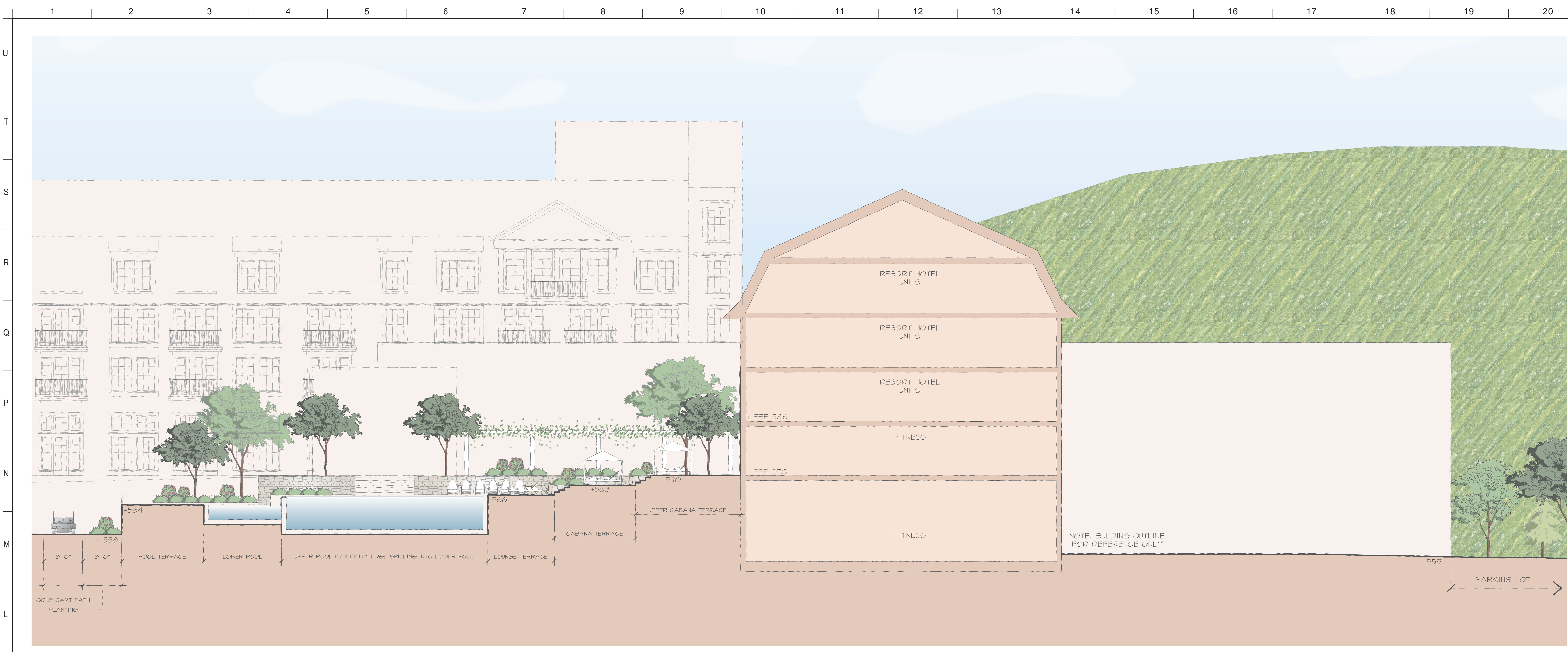
K1 SECTION THROUGH HOTEL POOL SCALE: 1/8" = 1'-0"
