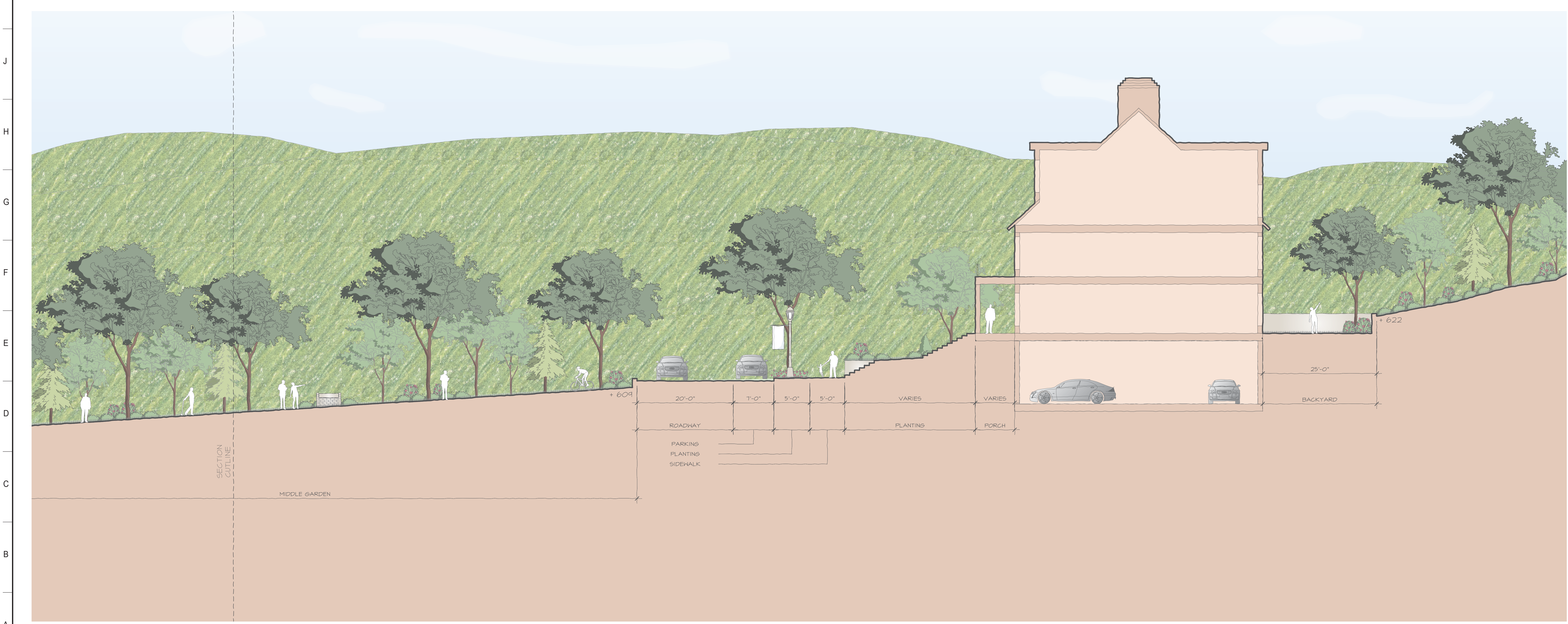
A1 SECTION THROUGH SHARED GARDENS SCALE: 1/8" = 1'-0"
